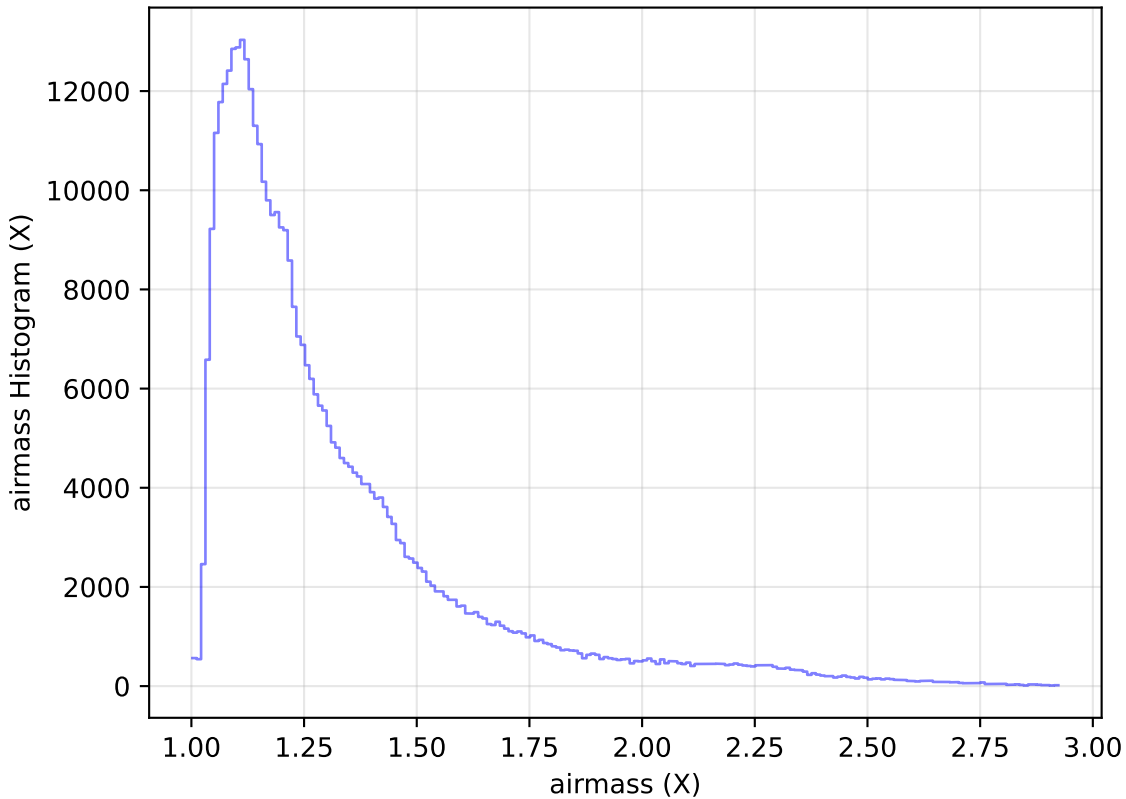
too_elab_r256_d2_gz_v3.4_10yrs WFD z band: airmass Histogram
