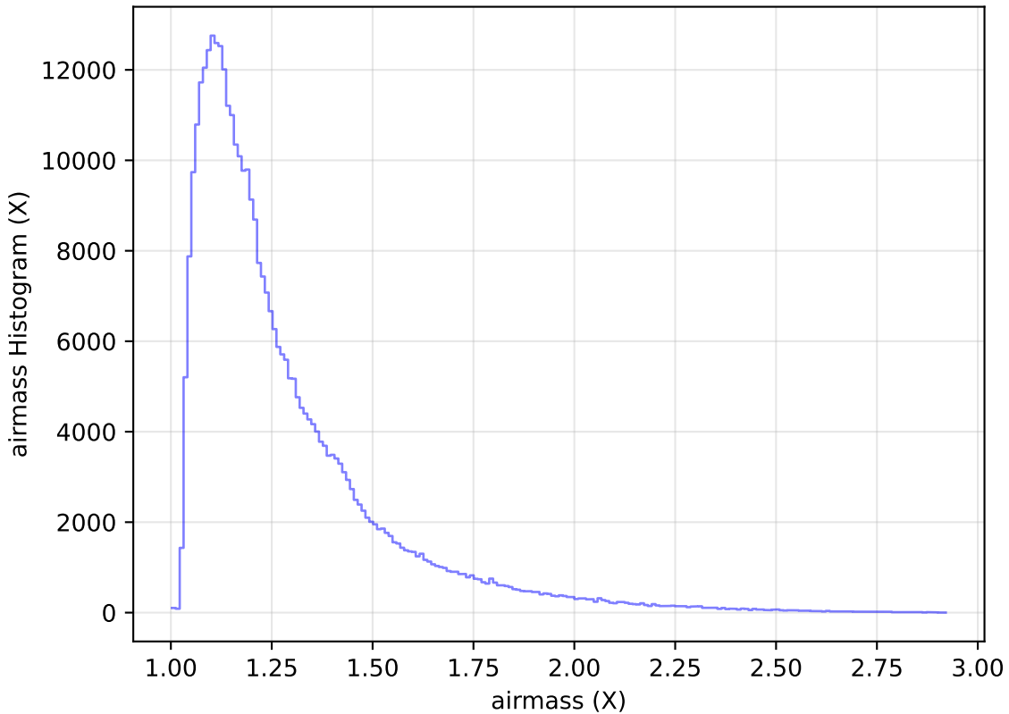
too_elab_r256_d2_gz_v3.4_10yrs WFD y band: airmass Histogram
