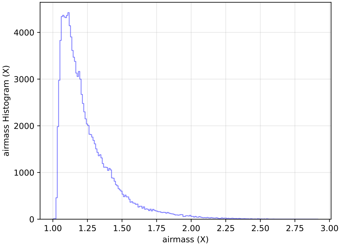
too_elab_r256_d2_gz_v3.4_10yrs WFD u band: airmass Histogram
