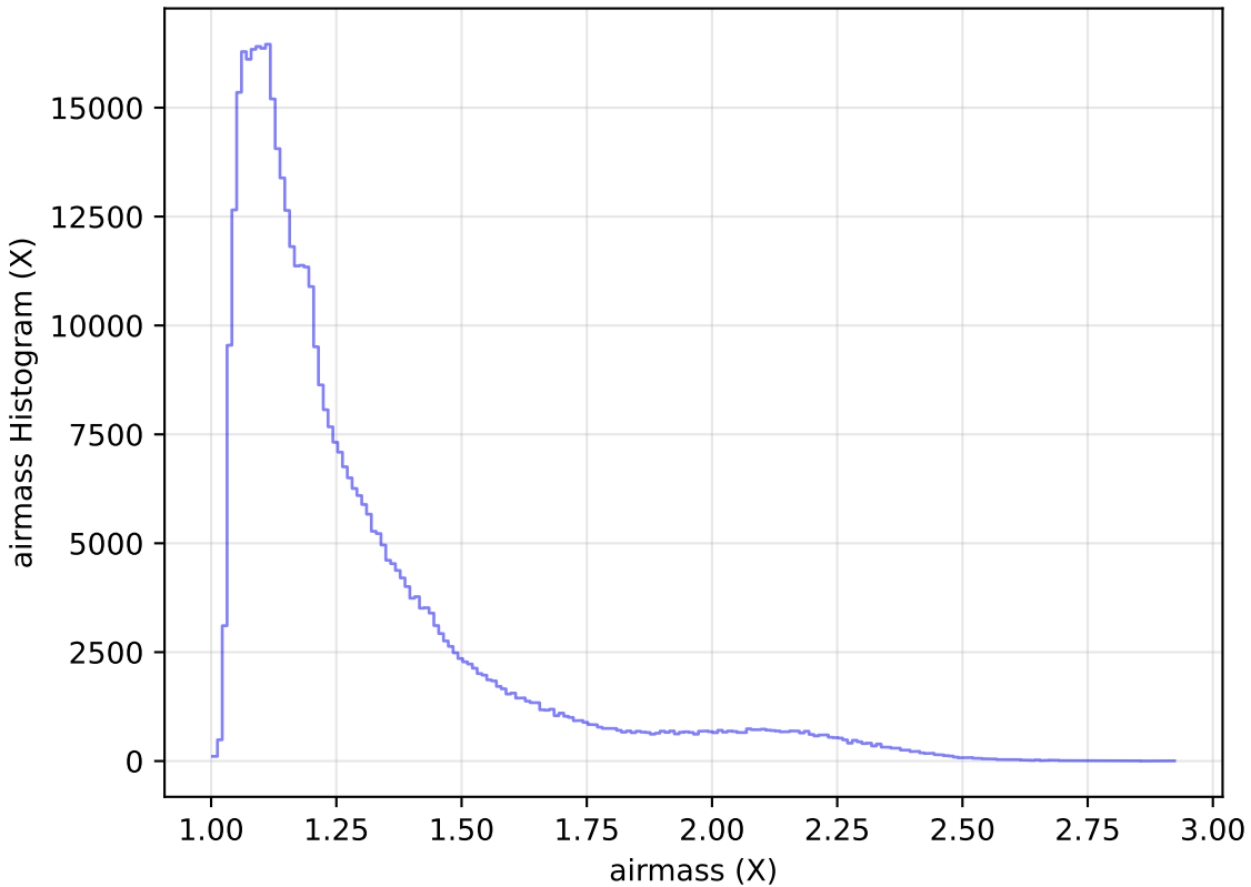
too_elab_r256_d2_gz_v3.4_10yrs WFD r band: airmass Histogram
