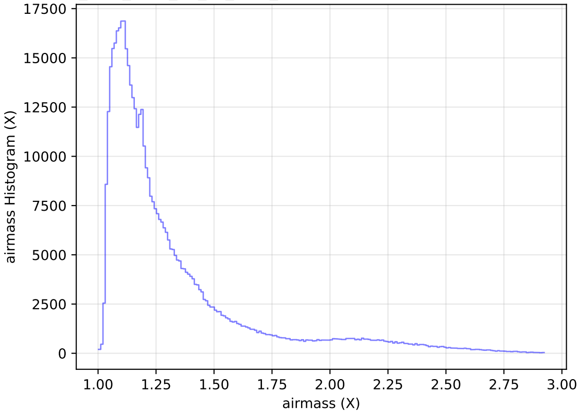
too_elab_r256_d2_gz_v3.4_10yrs WFD i band: airmass Histogram
