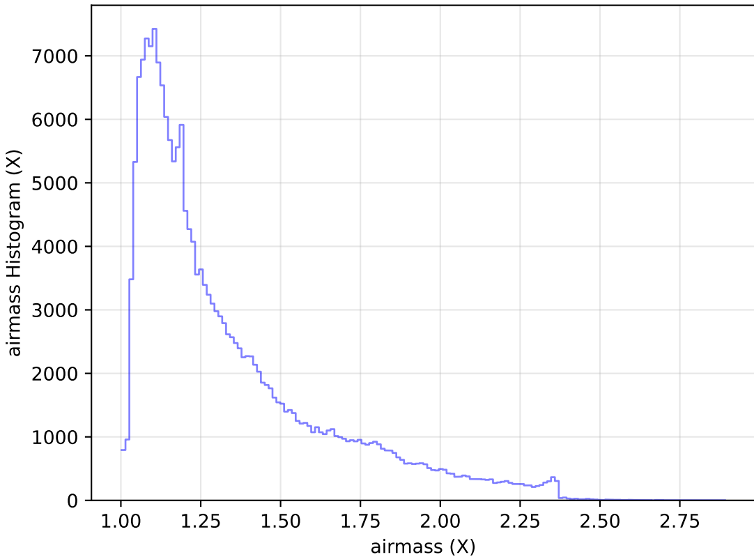
too_elab_r256_d2_gz_v3.4_10yrs WFD g band: airmass Histogram
