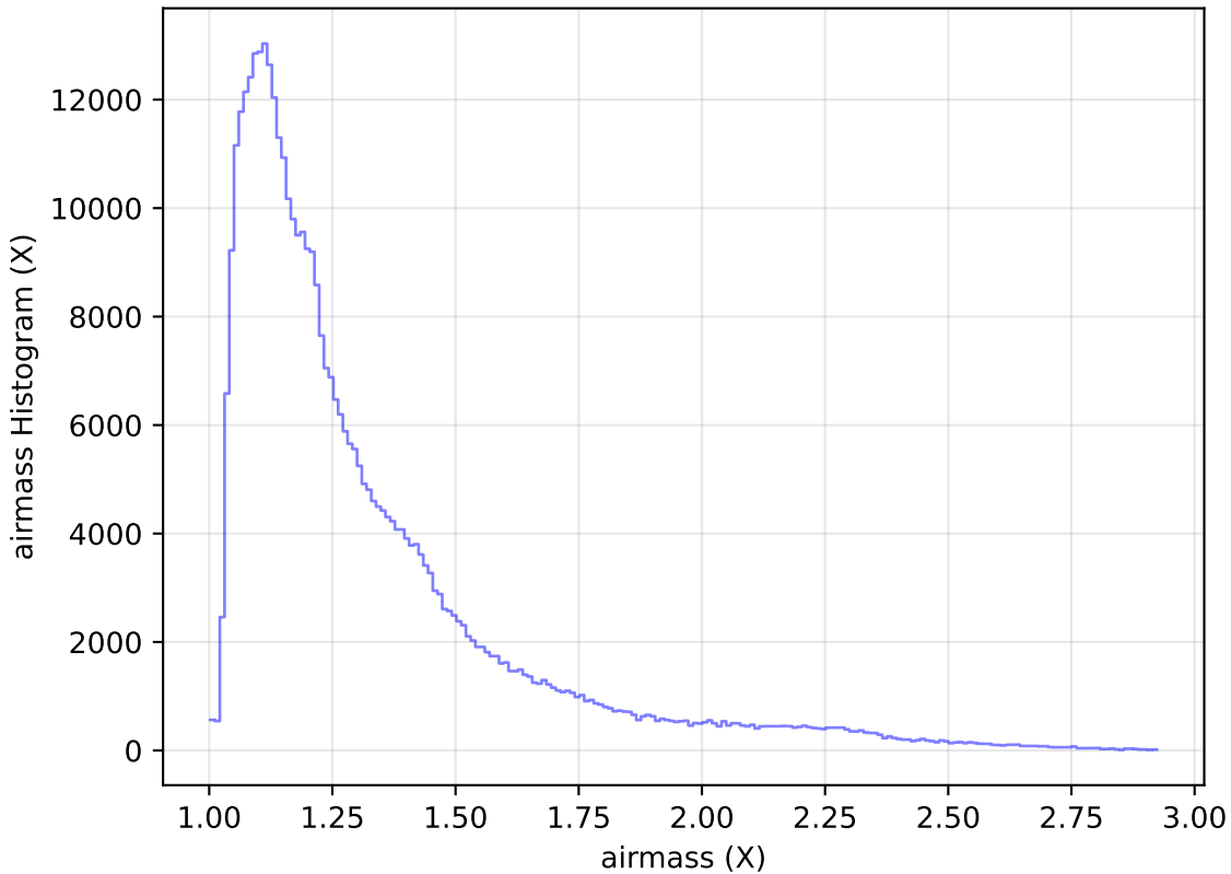
too_elab_r256_d2_gz_v3.4_10yrs All sky z band: airmass Histogram
