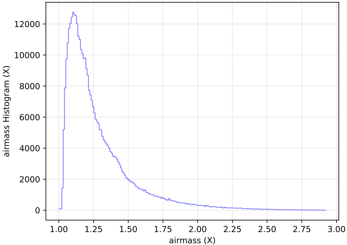
too_elab_r256_d2_gz_v3.4_10yrs All sky y band: airmass Histogram
