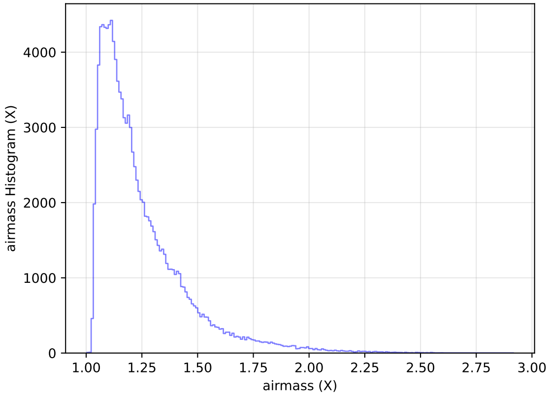
too_elab_r256_d2_gz_v3.4_10yrs All sky u band: airmass Histogram
