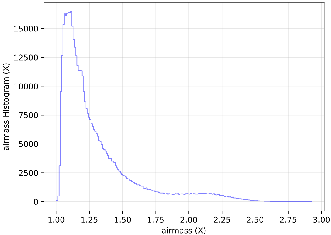
too_elab_r256_d2_gz_v3.4_10yrs All sky r band: airmass Histogram
