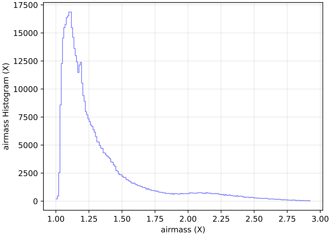
too_elab_r256_d2_gz_v3.4_10yrs All sky i band: airmass Histogram
