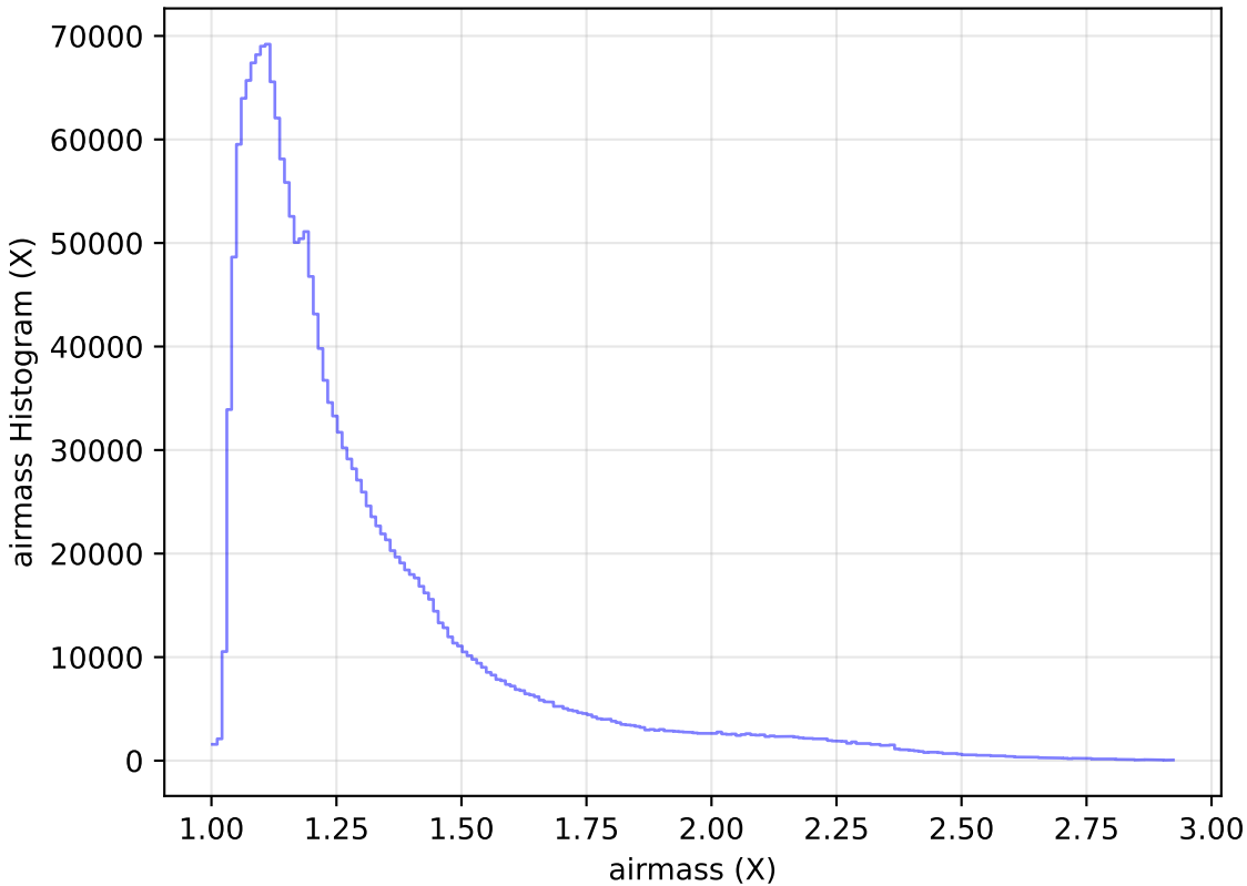
too_elab_r256_d2_gz_v3.4_10yrs All sky all bands: airmass Histogram
