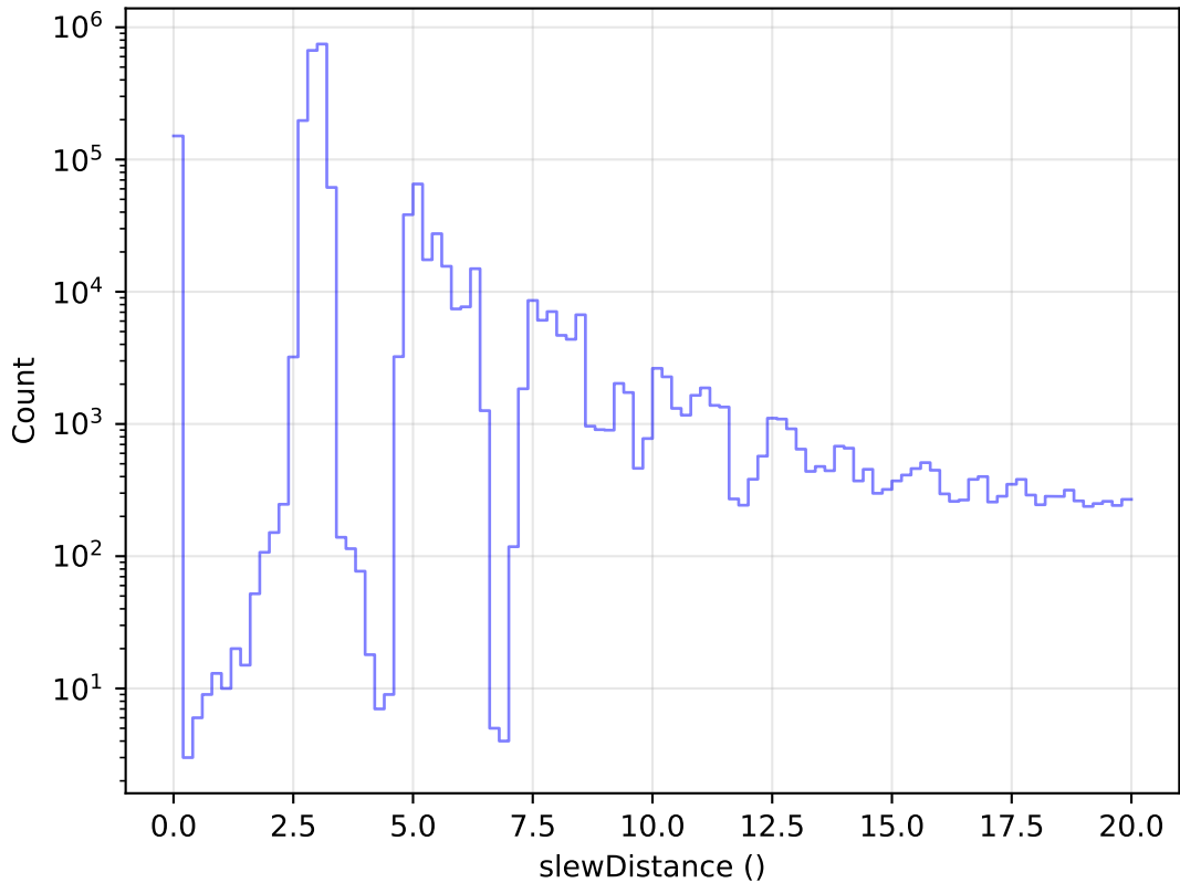
too_elab_r256_d2_gz_v3.4_10yrs All visits: Zoom Slew Distance Histogram
