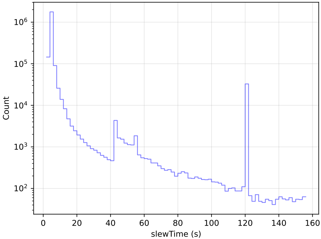
too_elab_r256_d2_gz_v3.4_10yrs All visits: Slew Time Histogram
