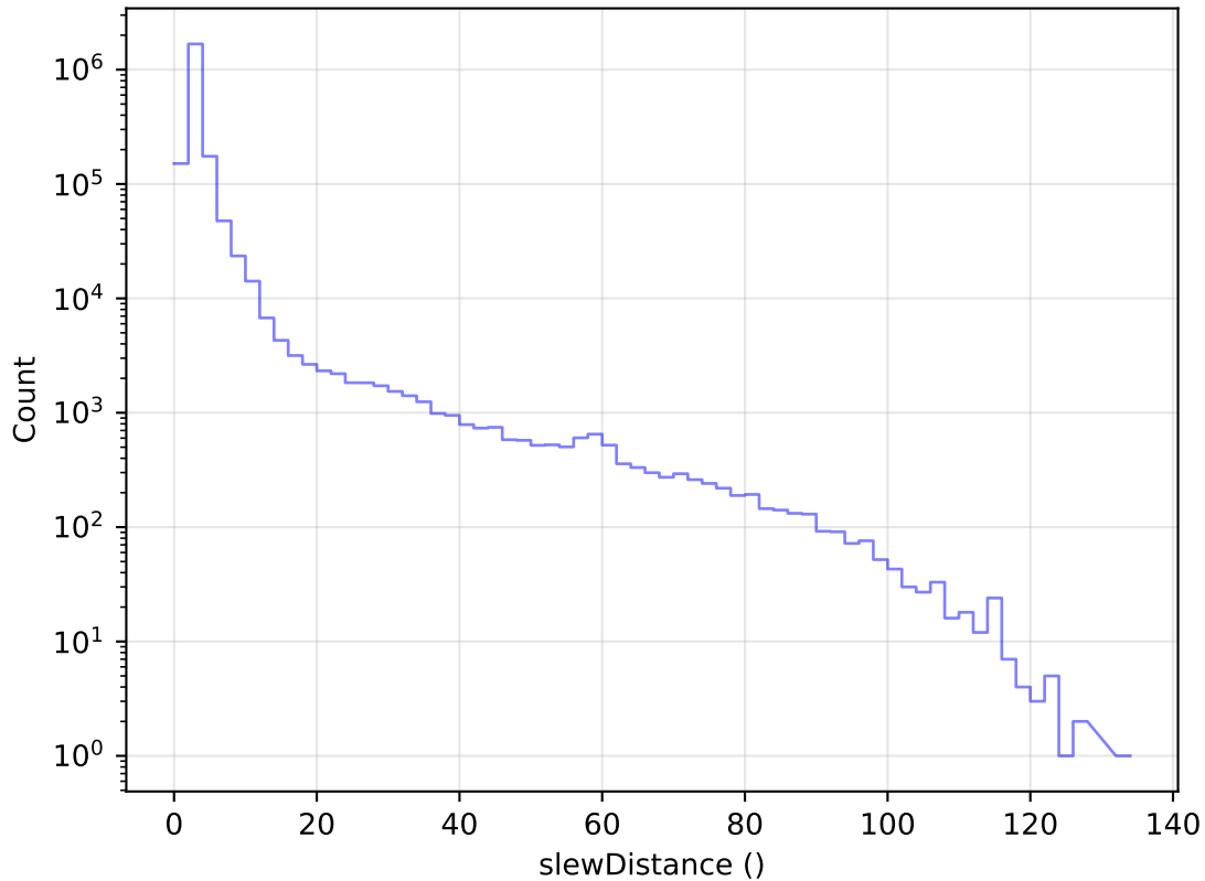
too_elab_r256_d2_gz_v3.4_10yrs All visits: Slew Distance Histogram
