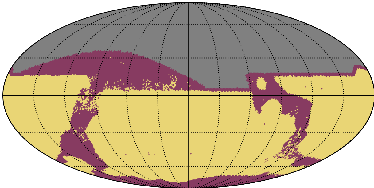
too_elab_r256_d2_gz_v3.4_10yrs All sky: RapidRevisits
