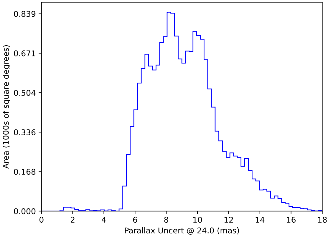
too_elab_r256_d2_gz_v3.4_10yrs WFD: Parallax Uncert @ 24.0
