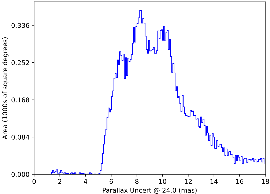
too_elab_r256_d2_gz_v3.4_10yrs All sky: Parallax Uncert @ 24.0
