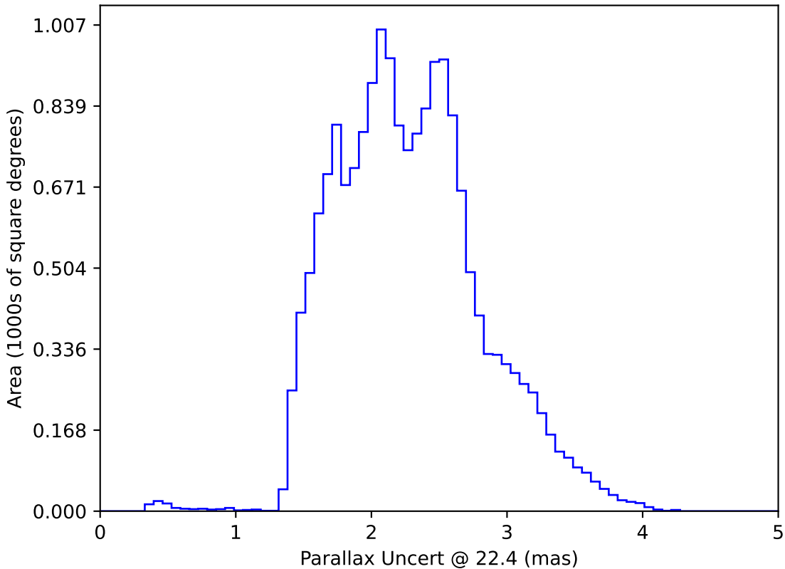
too_elab_r256_d2_gz_v3.4_10yrs WFD: Parallax Uncert @ 22.4
