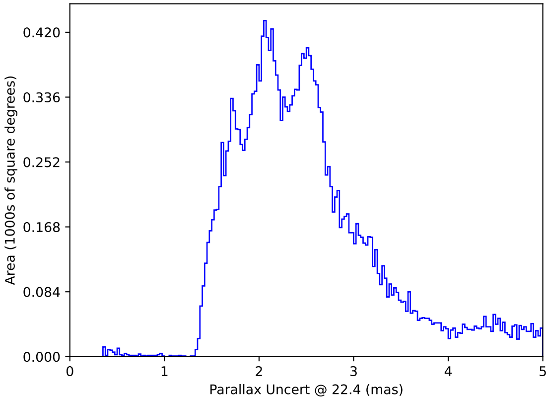
too_elab_r256_d2_gz_v3.4_10yrs All sky: Parallax Uncert @ 22.4
