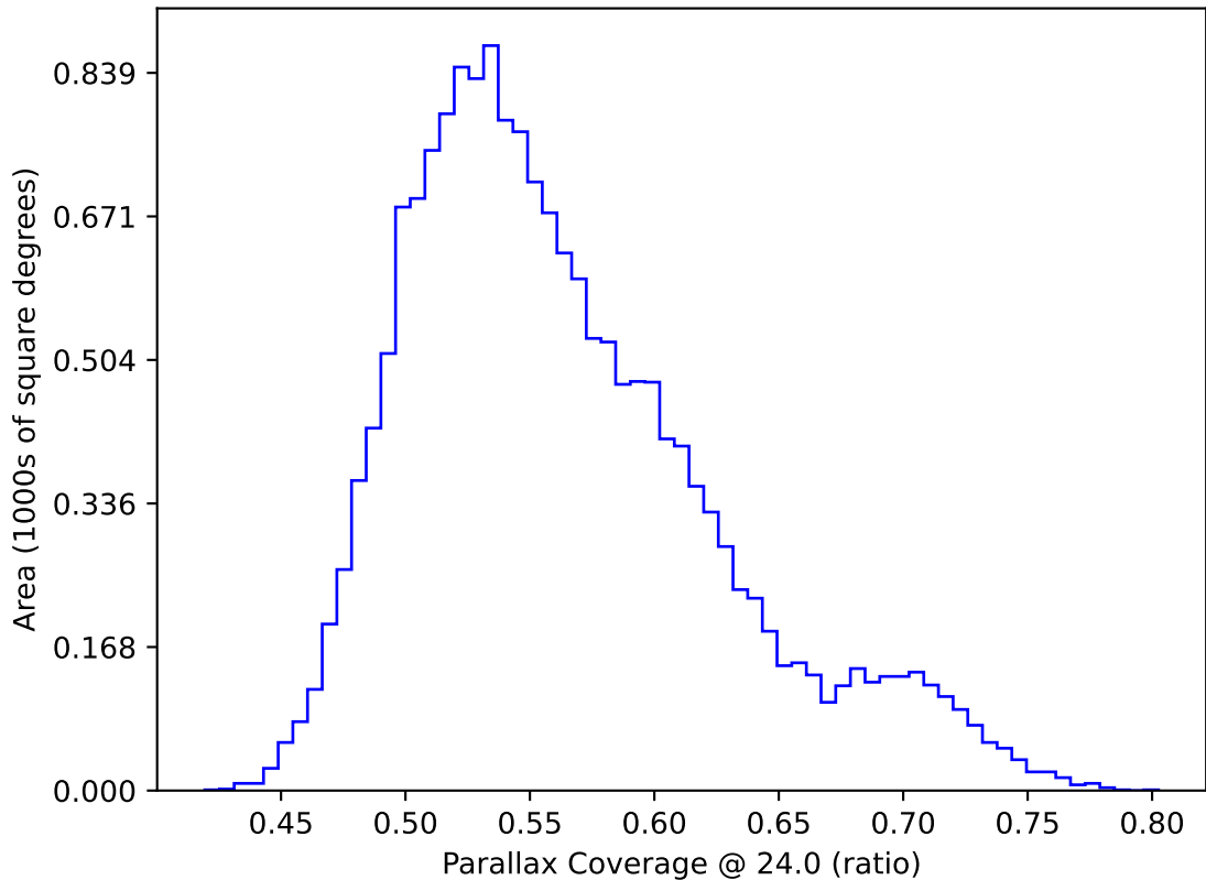
too_elab_r256_d2_gz_v3.4_10yrs WFD: Parallax Coverage @ 24.0
