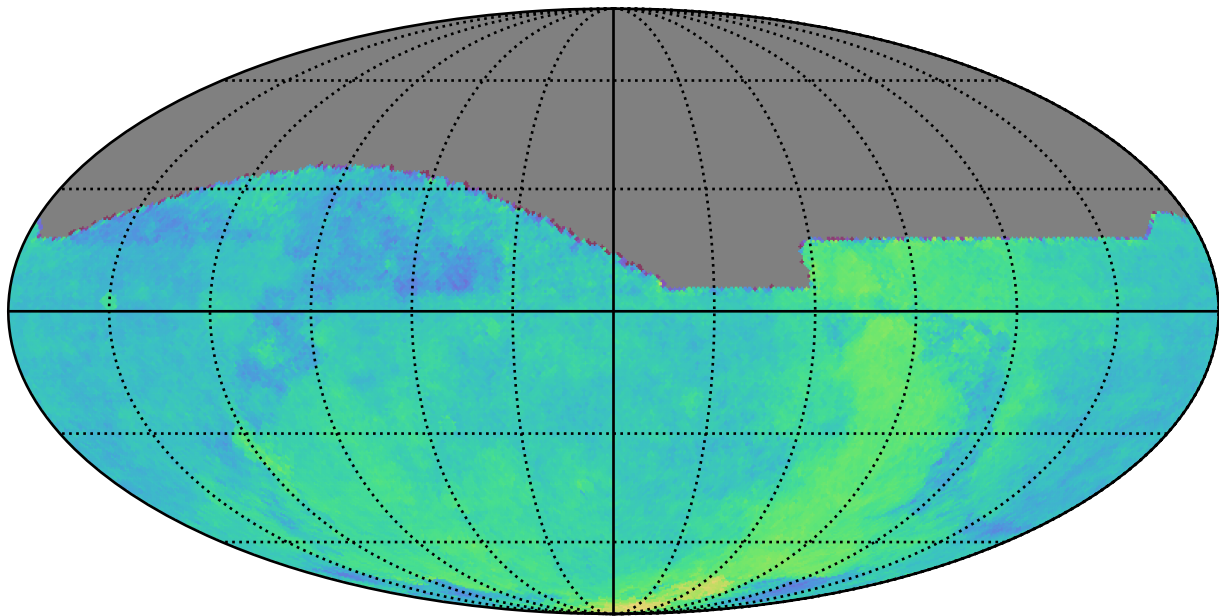
too_elab_r256_d2_gz_v3.4_10yrs All sky: Parallax Coverage @ 24.0
