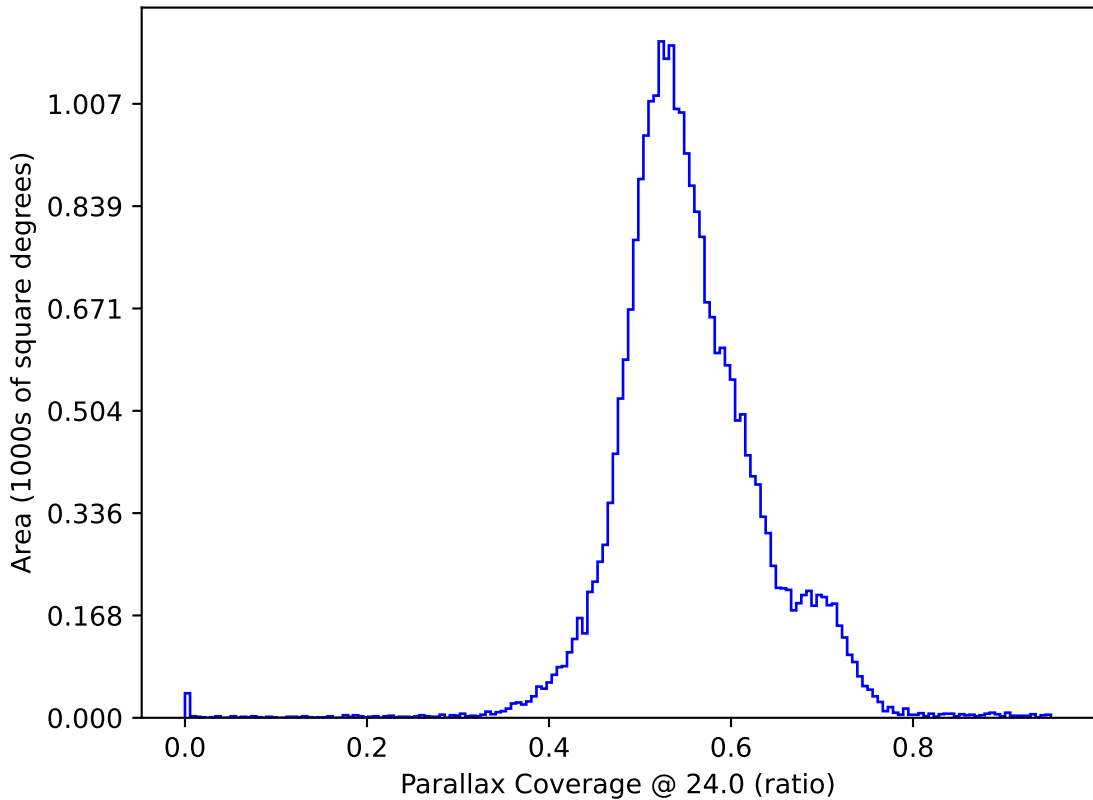
too_elab_r256_d2_gz_v3.4_10yrs All sky: Parallax Coverage @ 24.0
