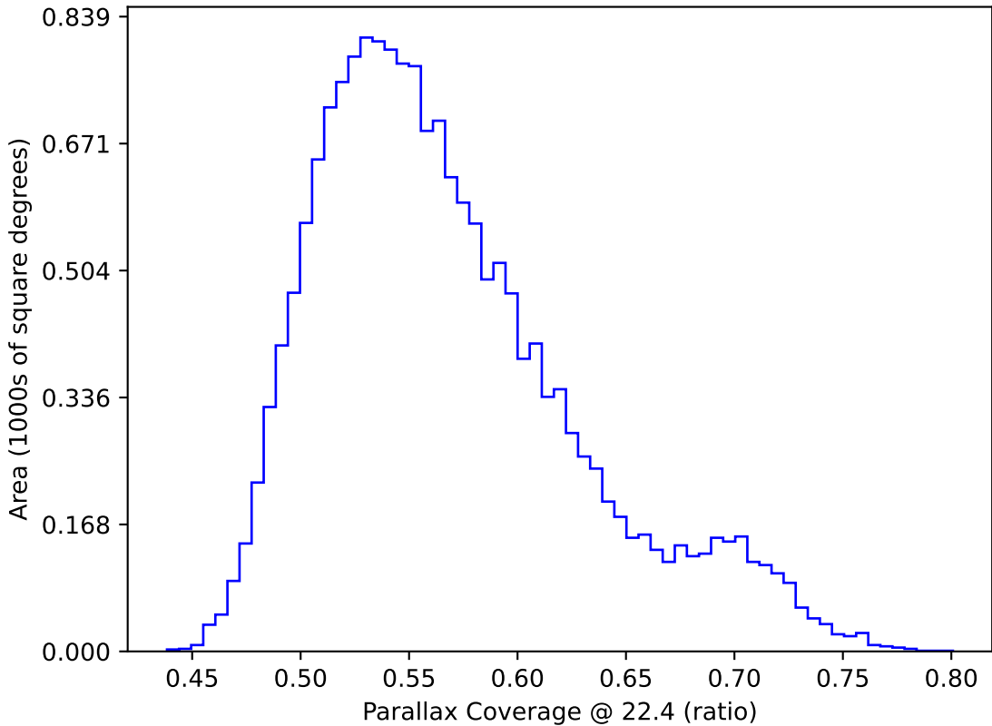
too_elab_r256_d2_gz_v3.4_10yrs WFD: Parallax Coverage @ 22.4
