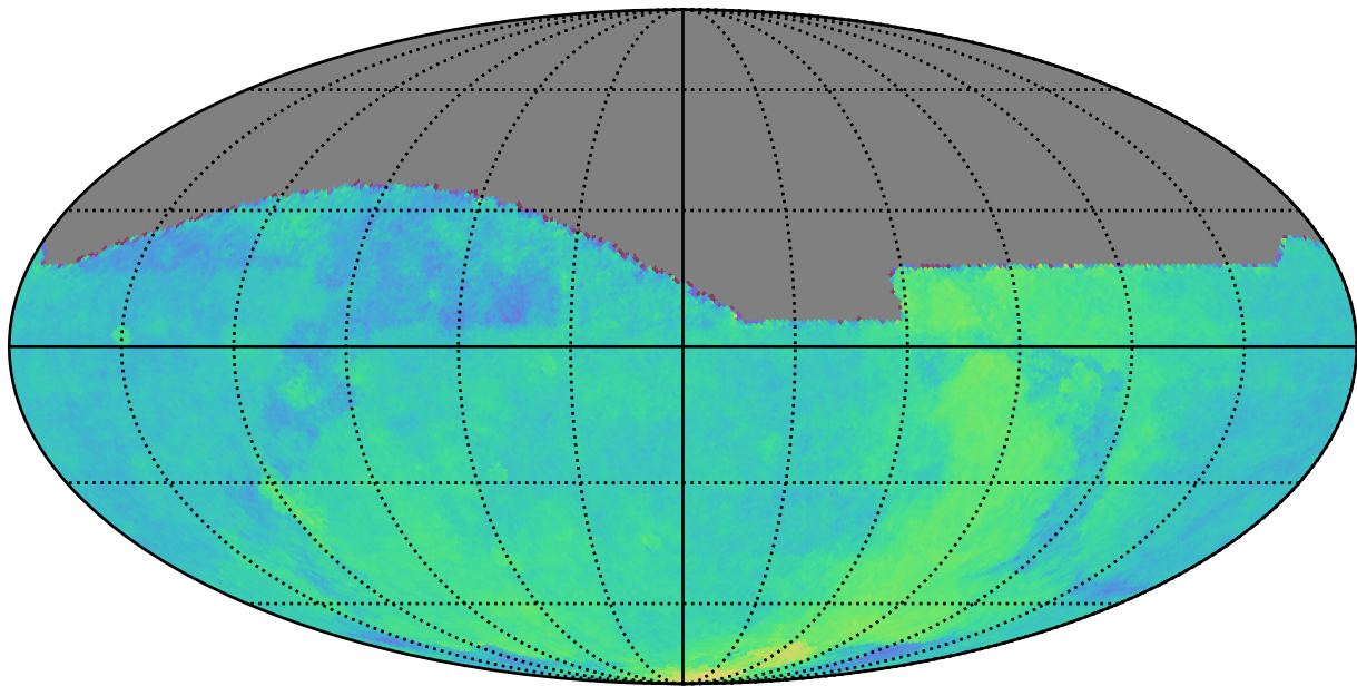
too_elab_r256_d2_gz_v3.4_10yrs All sky: Parallax Coverage @ 22.4
