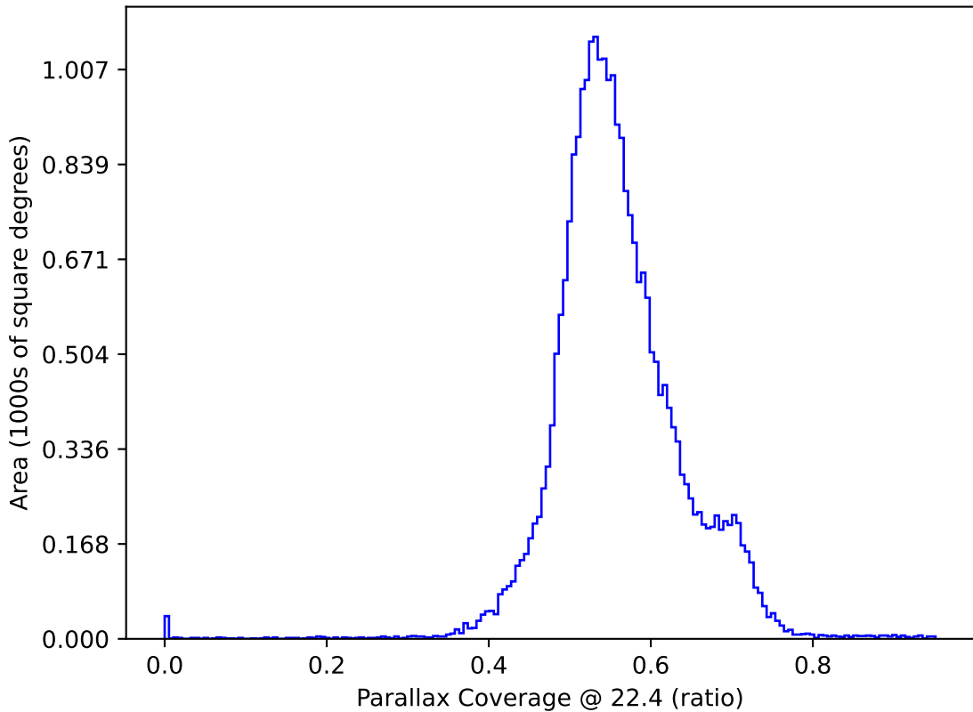
too_elab_r256_d2_gz_v3.4_10yrs All sky: Parallax Coverage @ 22.4
