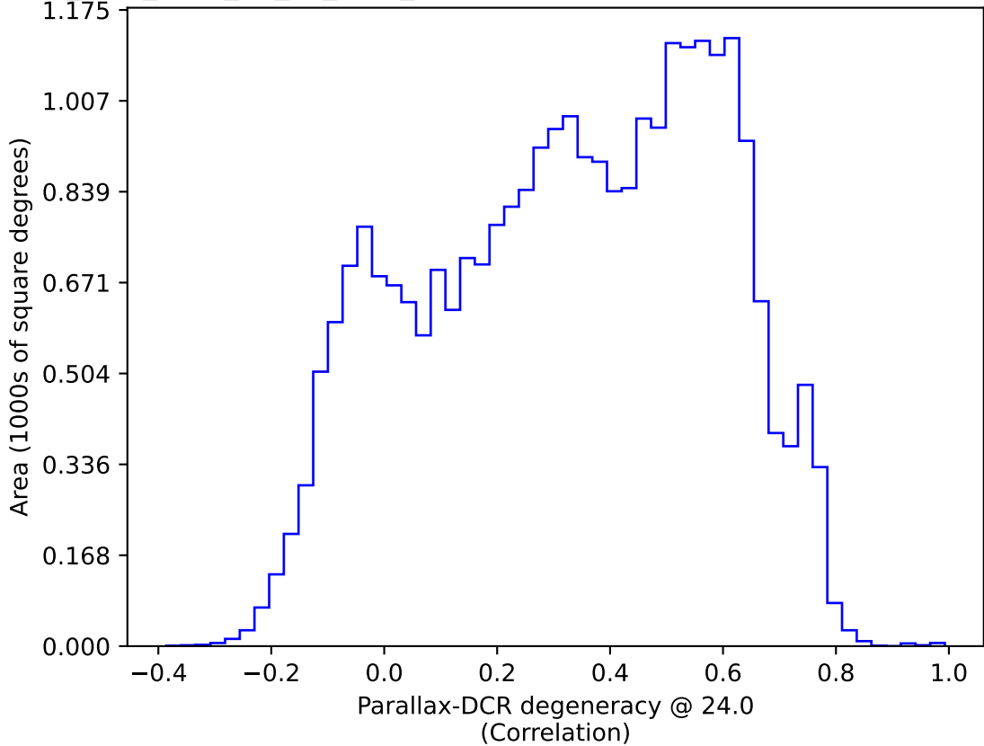
too_elab_r256_d2_gz_v3.4_10yrs All sky: Parallax-DCR degeneracy @ 24.0
