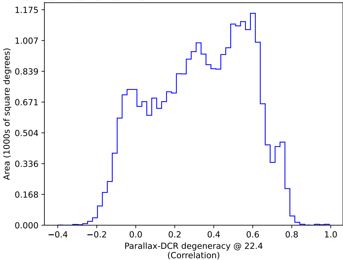
too_elab_r256_d2_gz_v3.4_10yrs All sky: Parallax-DCR degeneracy @ 22.4
