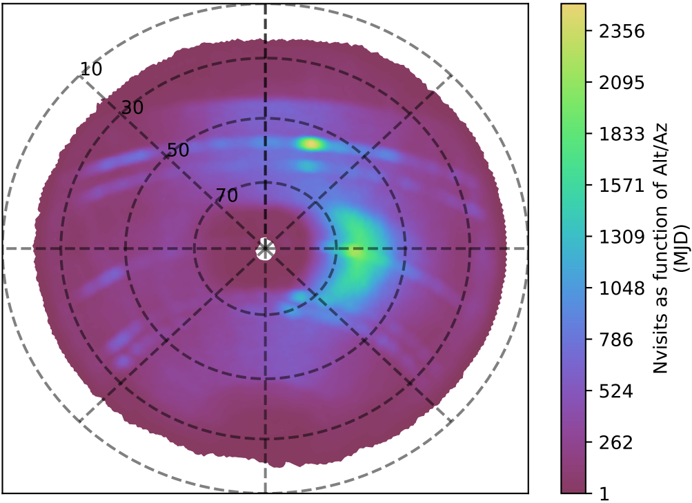
too_elab_r256_d2_gz_v3.4_10yrs z band: Nvisits as function of Alt/Az
