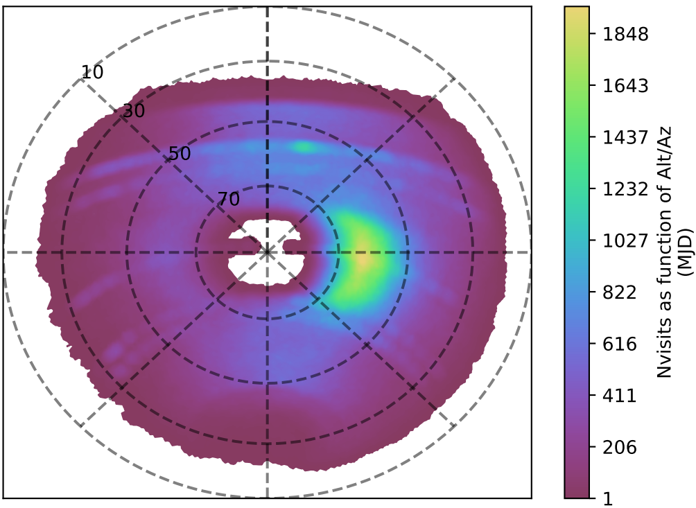
too_elab_r256_d2_gz_v3.4_10yrs y band: Nvisits as function of Alt/Az
