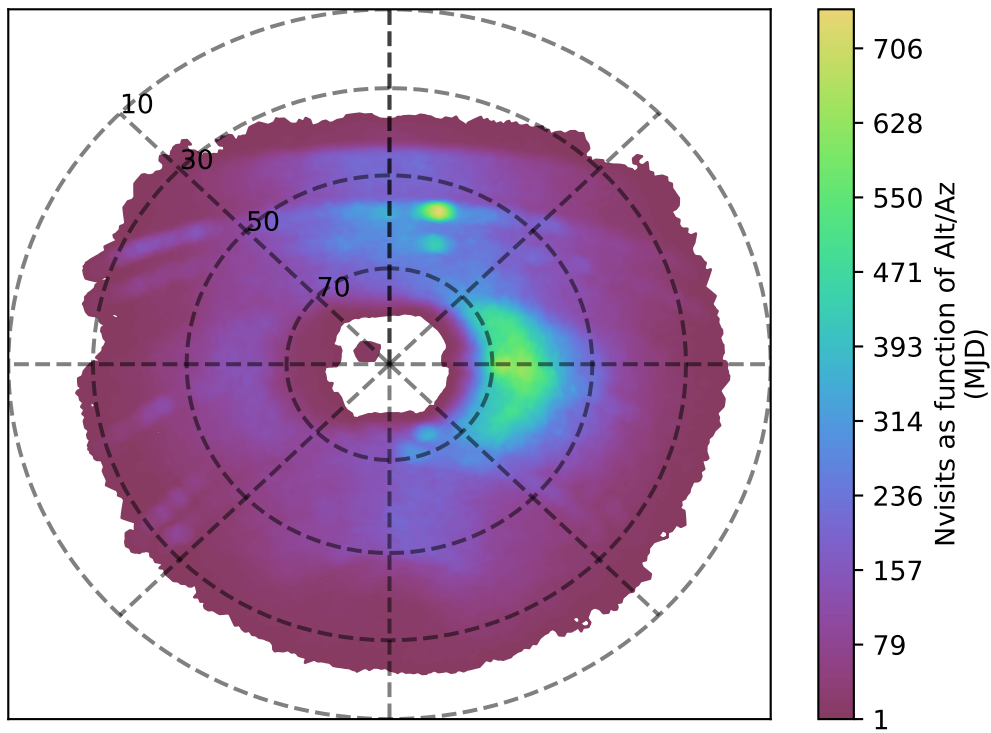
too_elab_r256_d2_gz_v3.4_10yrs u band: Nvisits as function of Alt/Az
