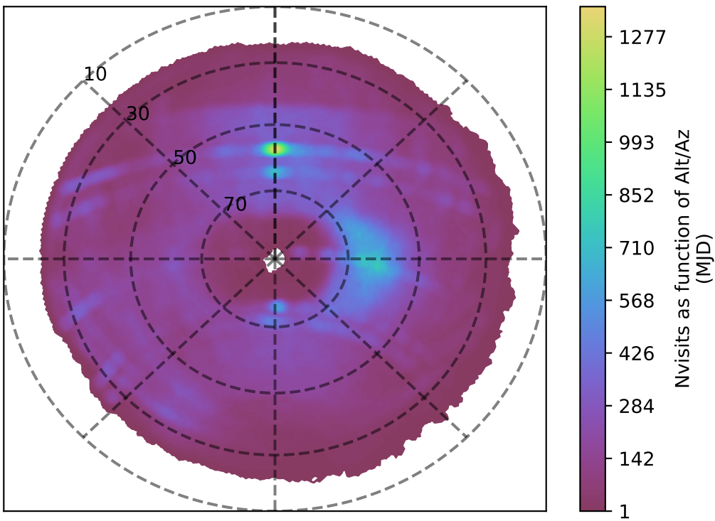
too_elab_r256_d2_gz_v3.4_10yrs g band: Nvisits as function of Alt/Az
