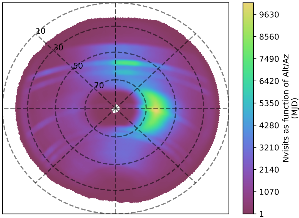
too_elab_r256_d2_gz_v3.4_10yrs all bands: Nvisits as function of Alt/Az
