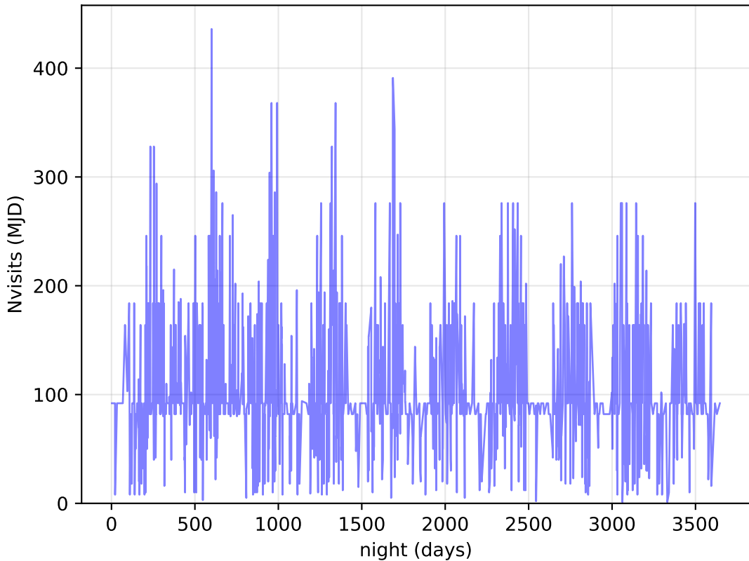
too_elab_r256_d2_gz_v3.4_10yrs DDF: Nvisits
