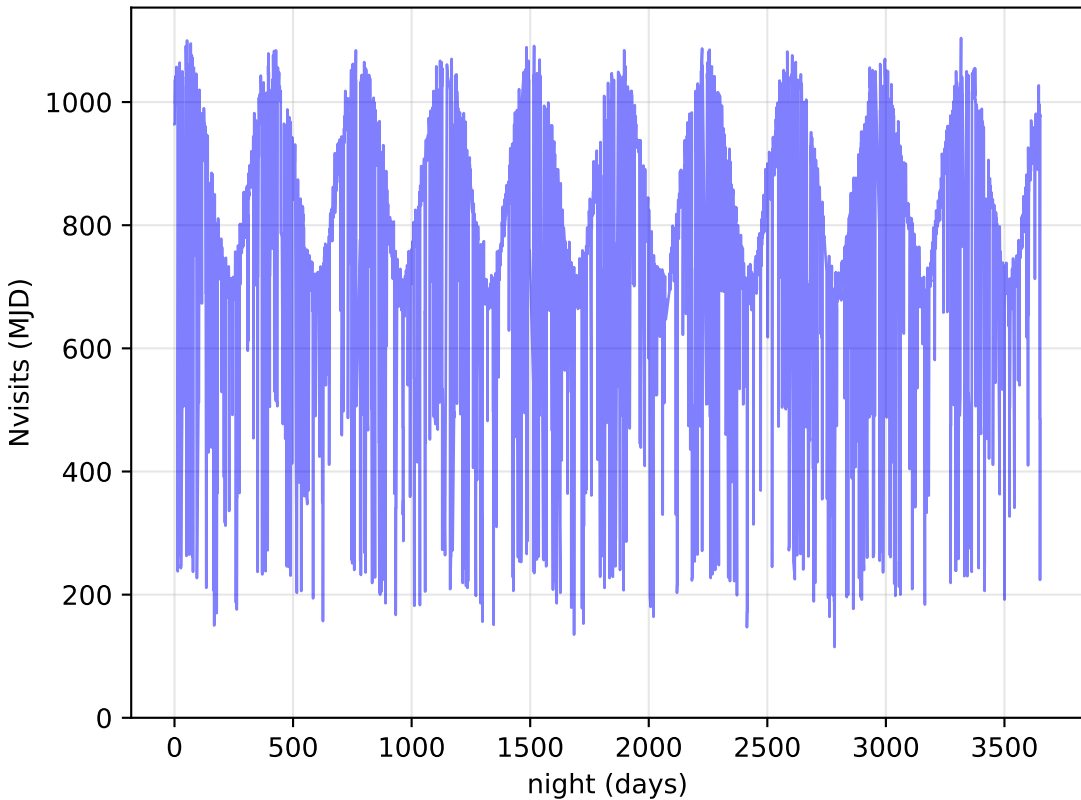
too_elab_r256_d2_gz_v3.4_10yrs All visits: Nvisits
