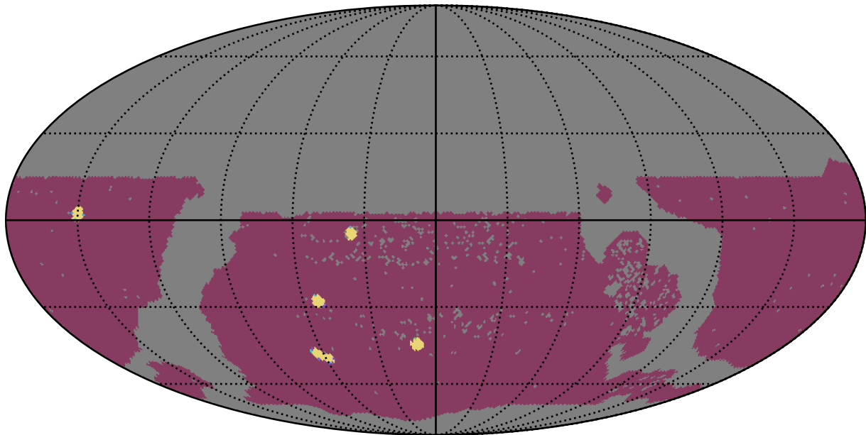
too_elab_r256_d2_gz_v3.4_10yrs WFD: NumberOfQuickRevisits
