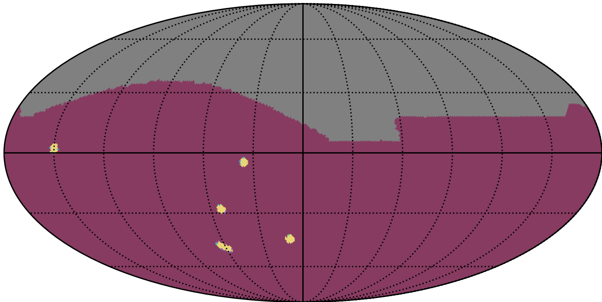
too_elab_r256_d2_gz_v3.4_10yrs All sky: NumberOfQuickRevisits
