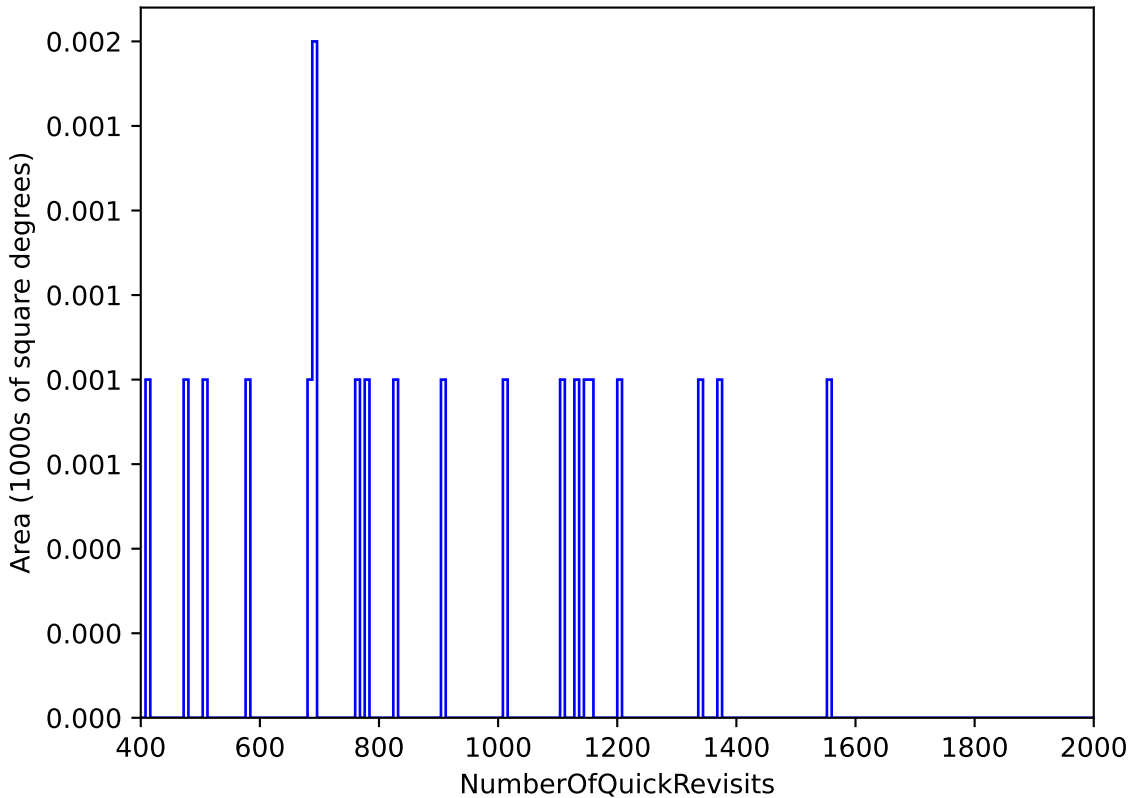
too_elab_r256_d2_gz_v3.4_10yrs All sky: NumberOfQuickRevisits
