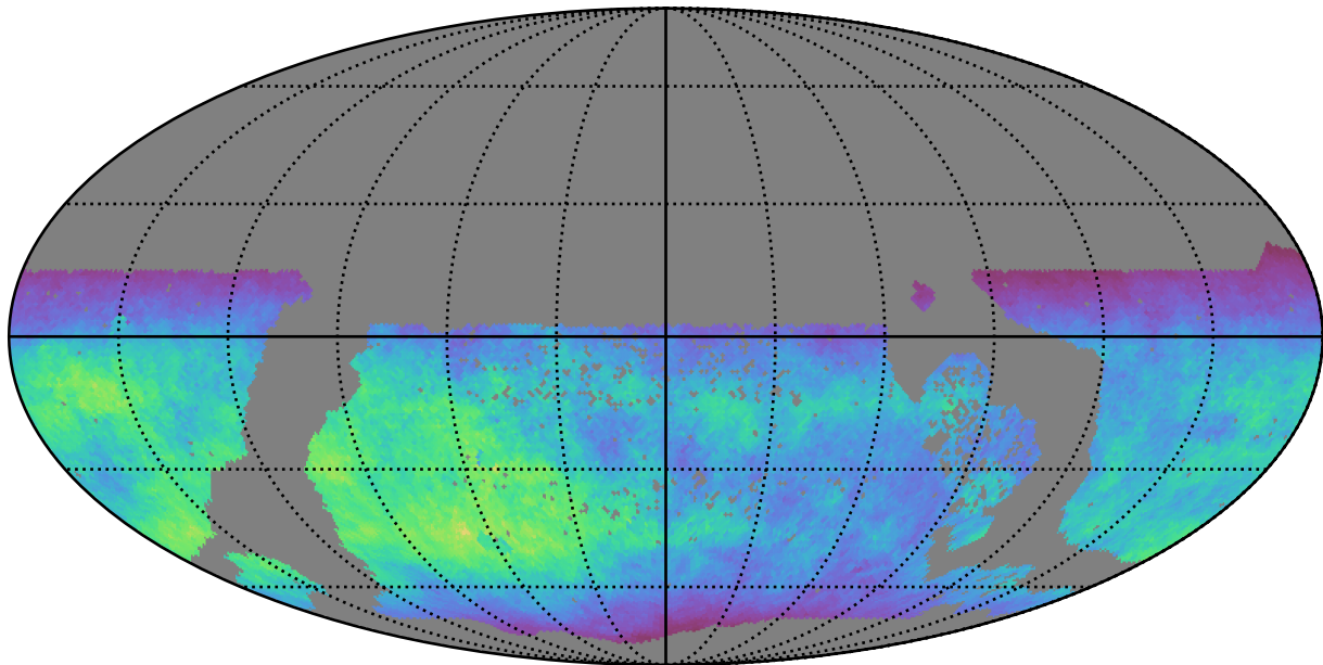
too_elab_r256_d2_gz_v3.4_10yrs WFD z band: Normalized Teff
