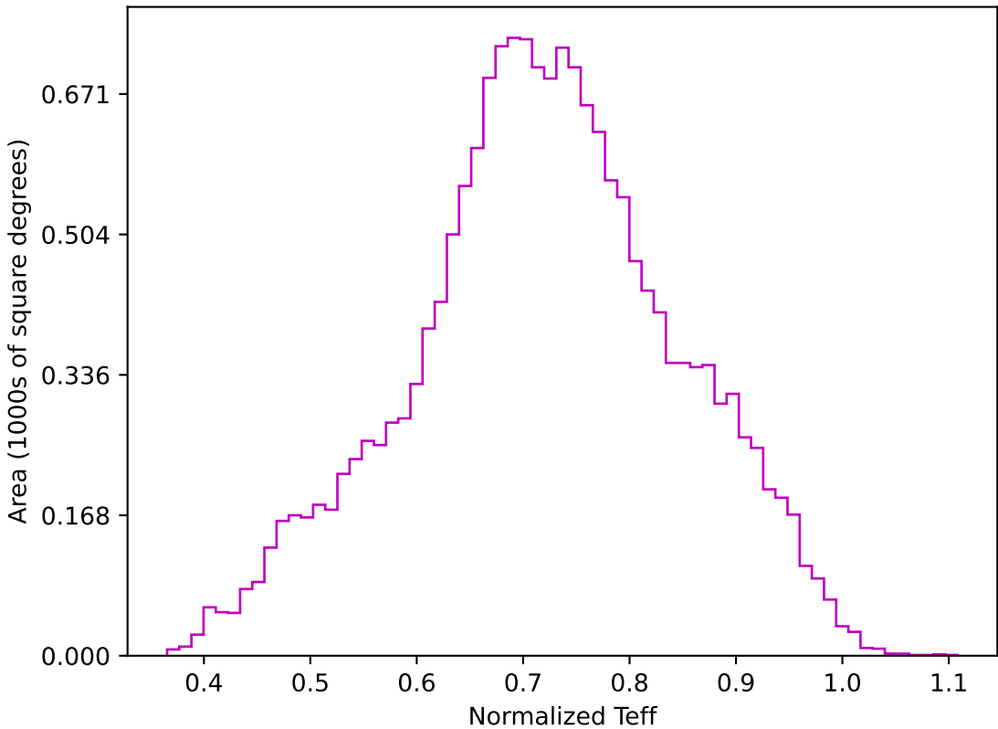
too_elab_r256_d2_gz_v3.4_10yrs WFD z band: Normalized Teff
