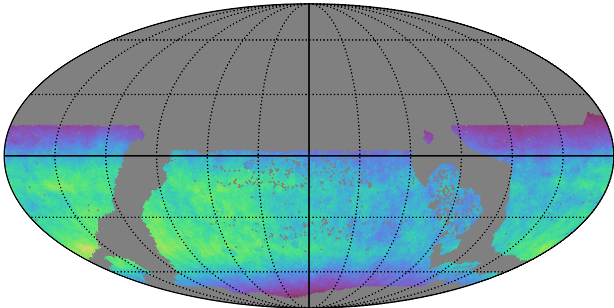
too_elab_r256_d2_gz_v3.4_10yrs WFD y band: Normalized Teff
