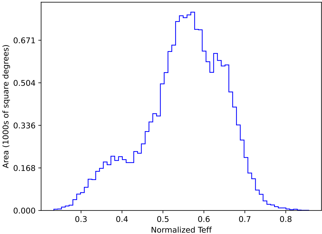
too_elab_r256_d2_gz_v3.4_10yrs WFD y band: Normalized Teff
