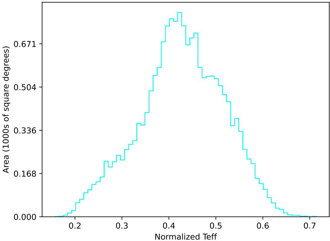
too_elab_r256_d2_gz_v3.4_10yrs WFD u band: Normalized Teff
