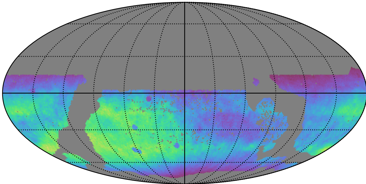
too_elab_r256_d2_gz_v3.4_10yrs WFD r band: Normalized Teff
