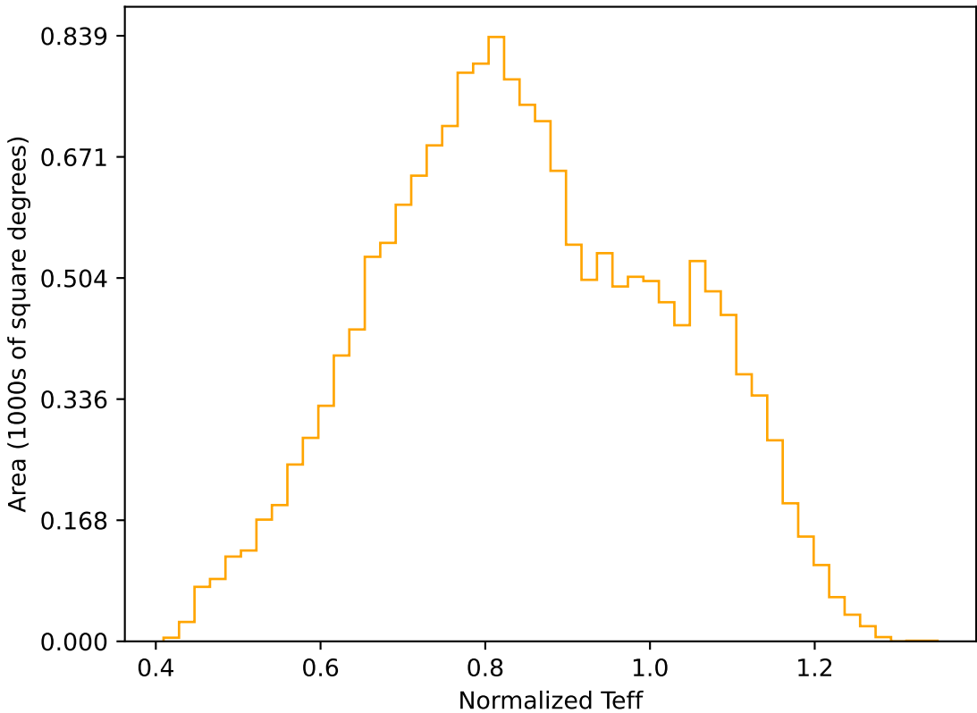
too_elab_r256_d2_gz_v3.4_10yrs WFD r band: Normalized Teff
