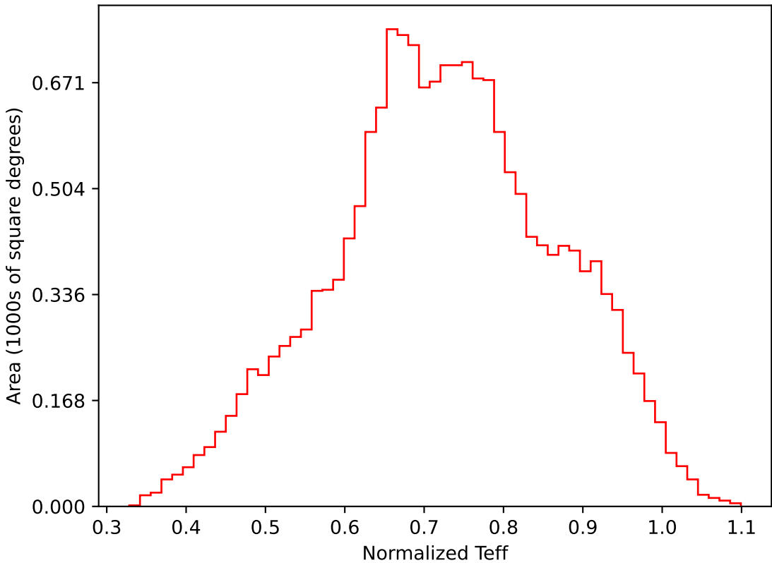
too_elab_r256_d2_gz_v3.4_10yrs WFD i band: Normalized Teff
