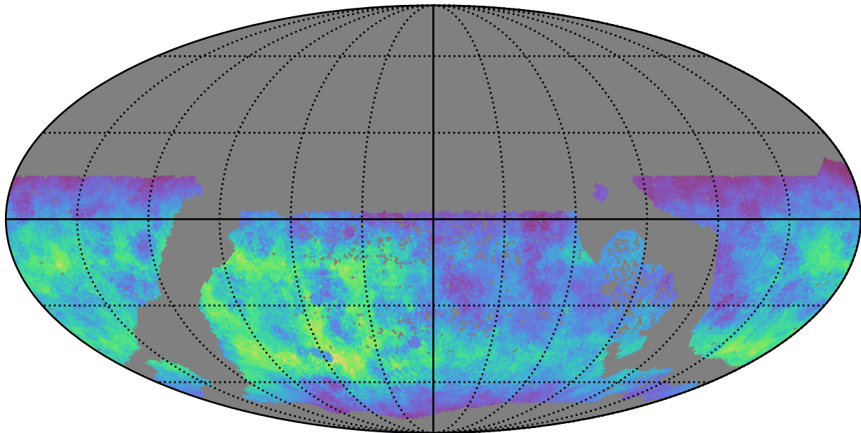
too_elab_r256_d2_gz_v3.4_10yrs WFD g band: Normalized Teff
