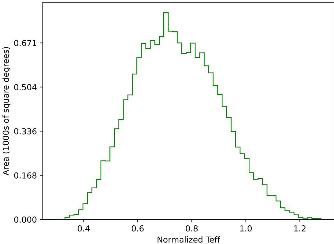
too_elab_r256_d2_gz_v3.4_10yrs WFD g band: Normalized Teff
