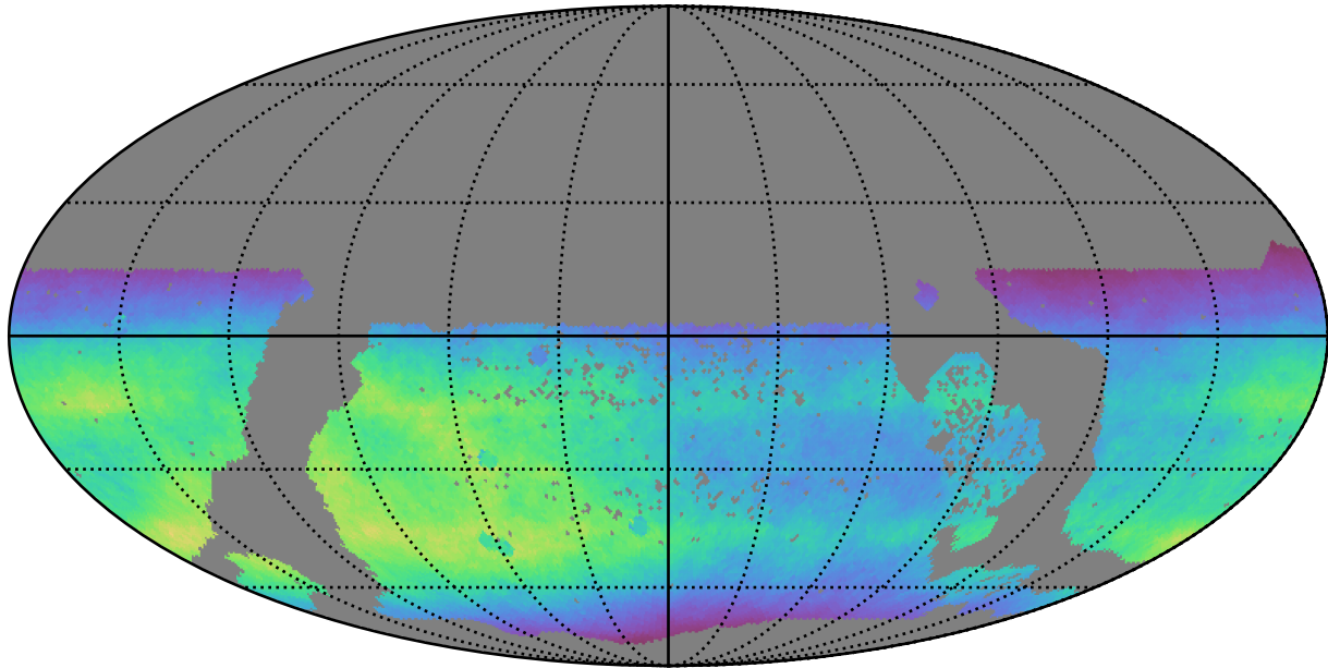
too_elab_r256_d2_gz_v3.4_10yrs WFD all bands: Normalized Teff
