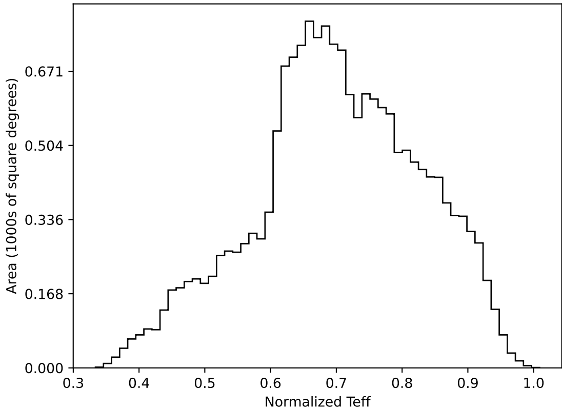
too_elab_r256_d2_gz_v3.4_10yrs WFD all bands: Normalized Teff
